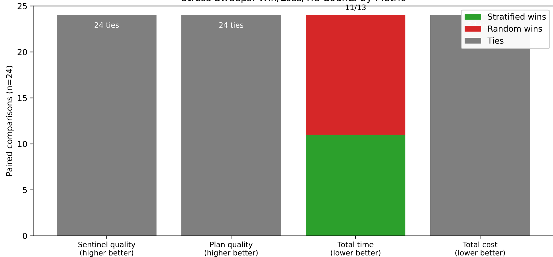
Stress Sweeps: Win/Loss/Tie Counts by Metric
