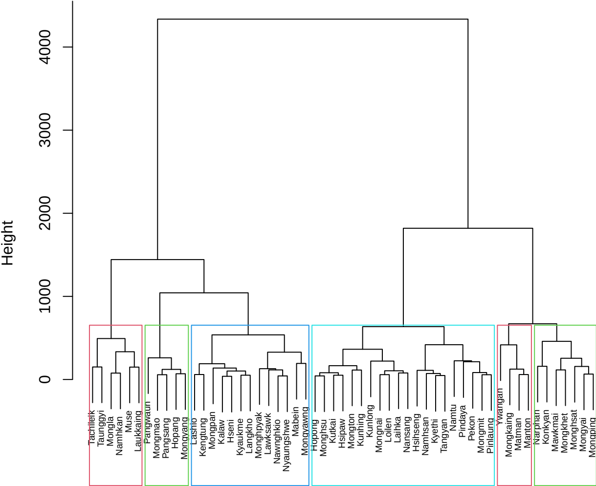
Cluster Dendrogram
