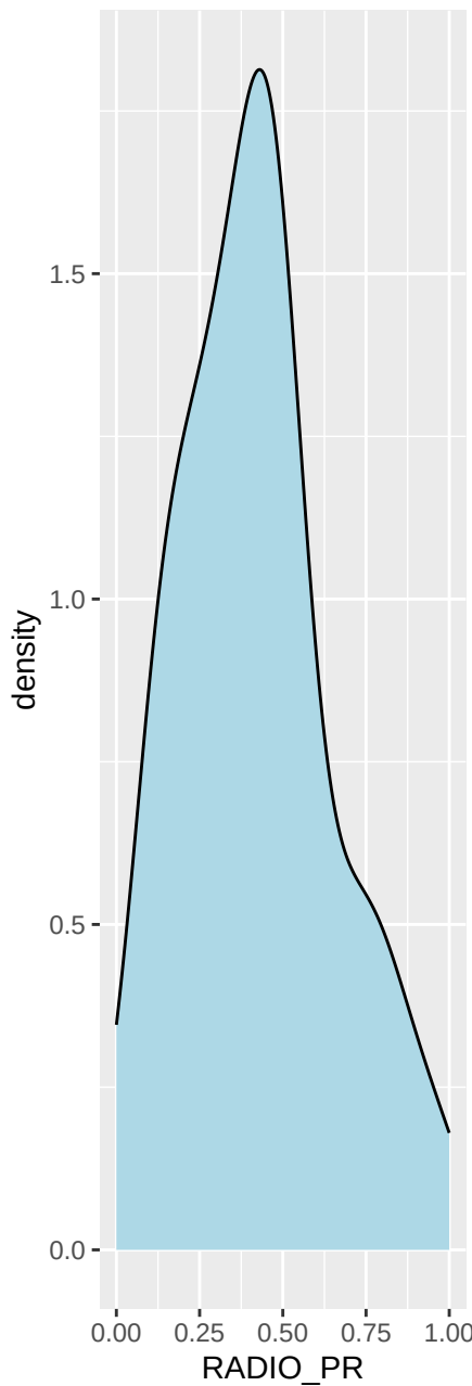
Min-Max Standardisati
