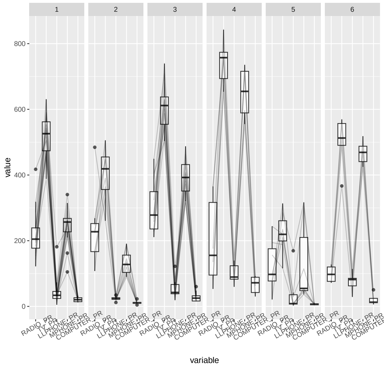
Multiple Parallel Coordinates Plots of ICT Variables by Cluster
