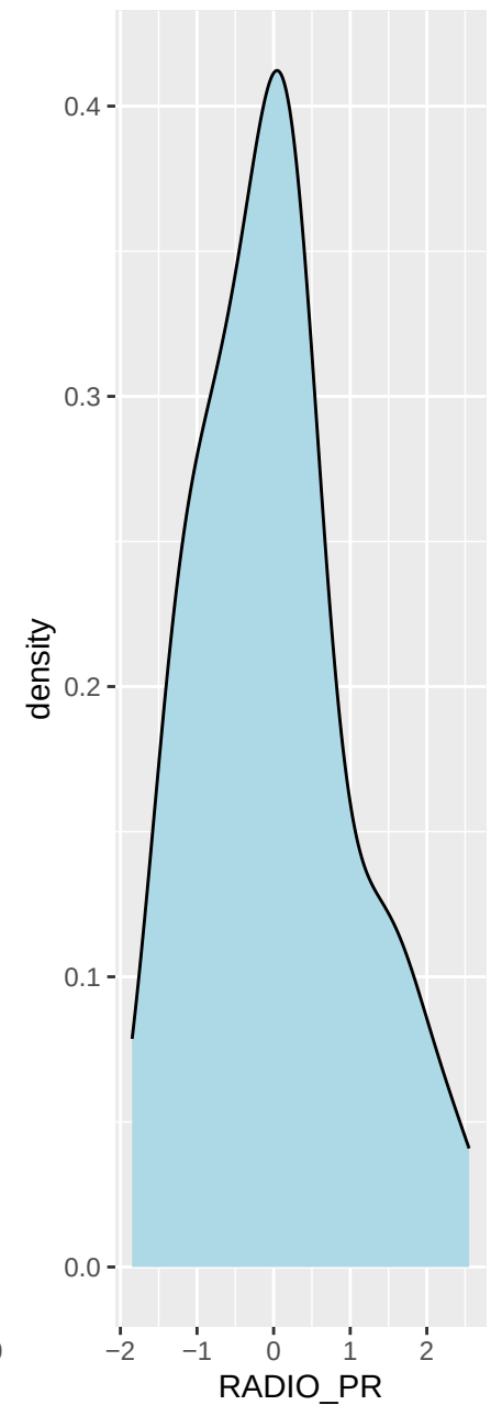
Z-score Standardisatio
