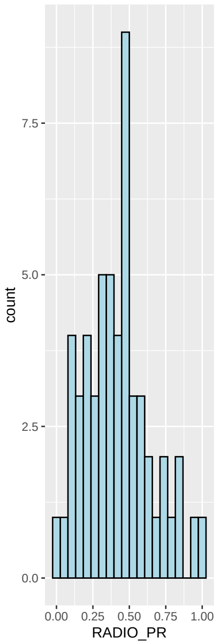
Min-Max Standardisati
