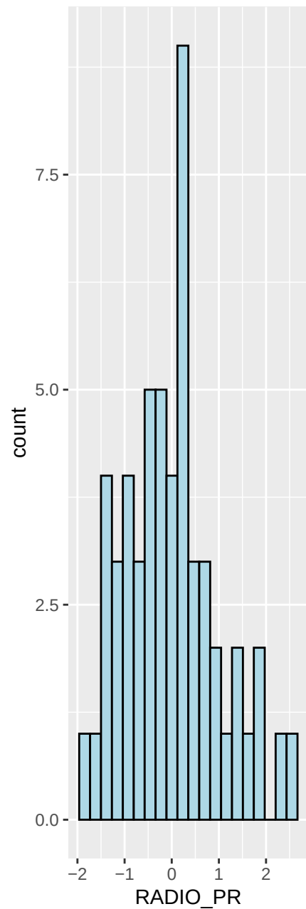
Z-score Standardisatio
