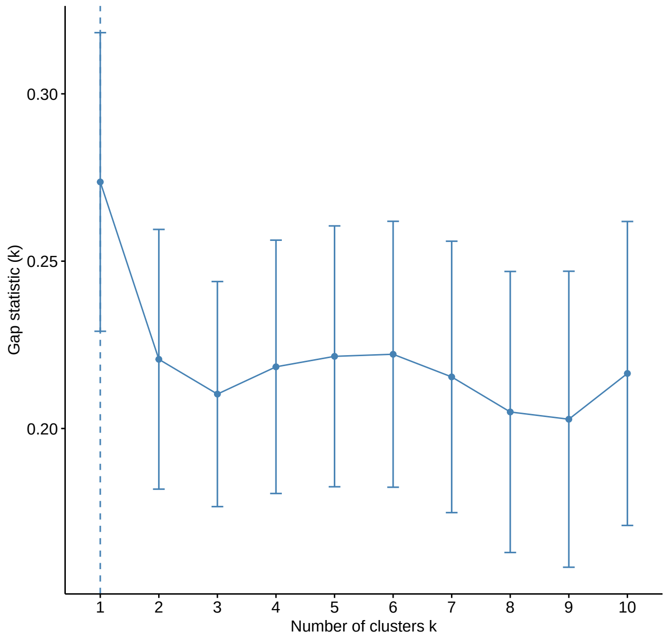
Optimal number of clusters (method = "gap_stat")
