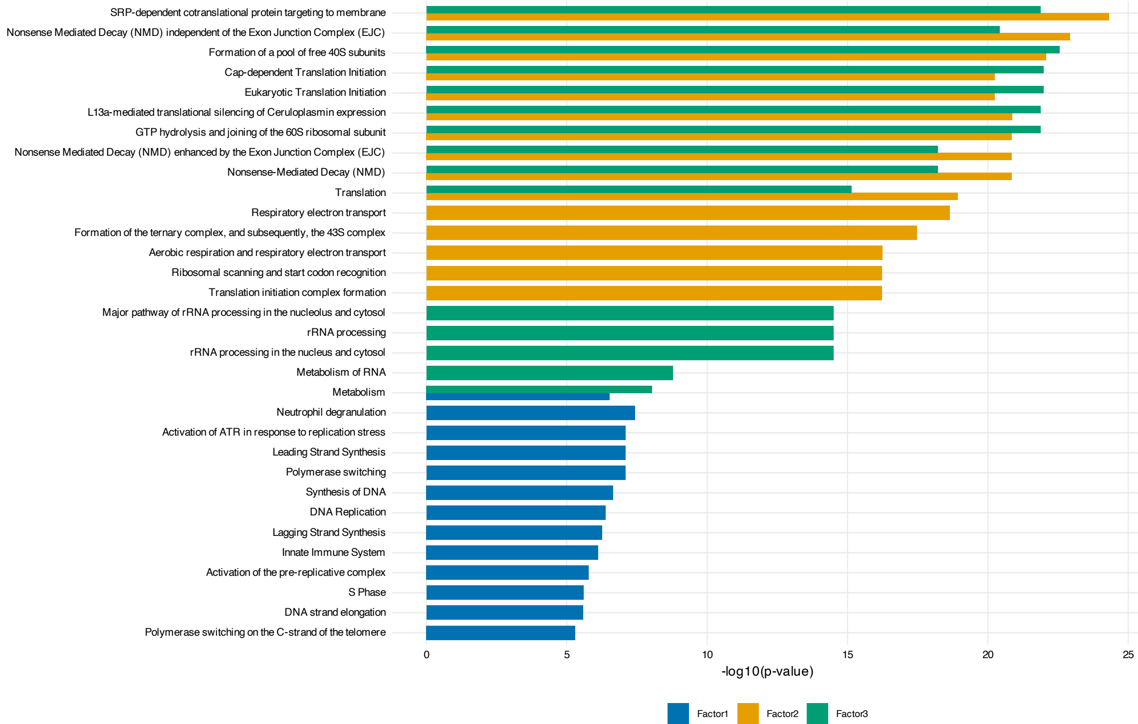
Reactome pathway enrichment per MEFISTO factor (top 15 by p-value)
