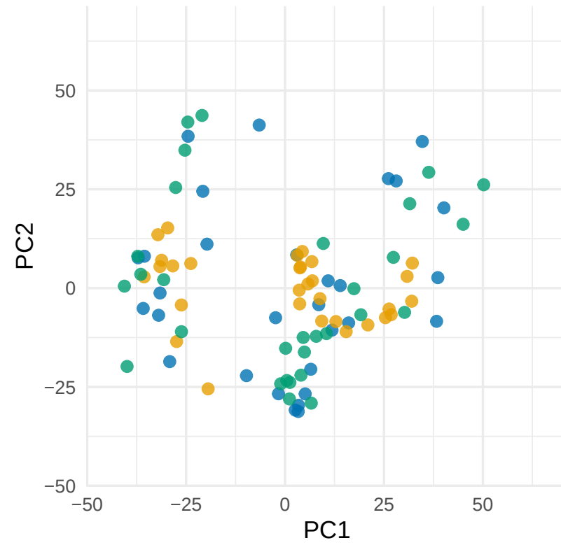
After ComBat
