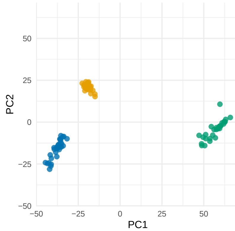
Before ComBat
