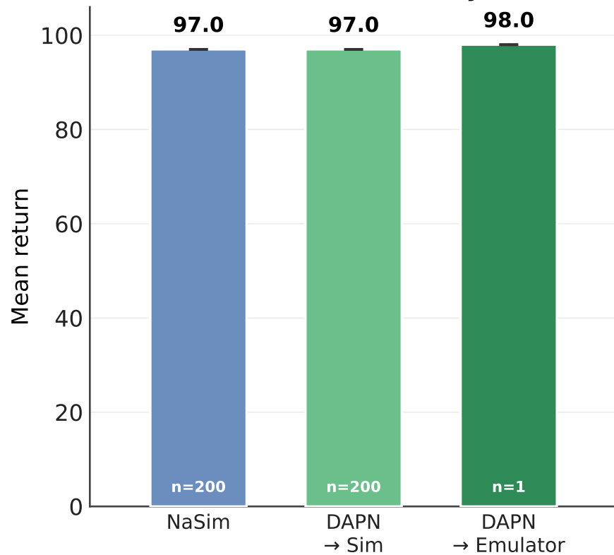
Solution efficiency
