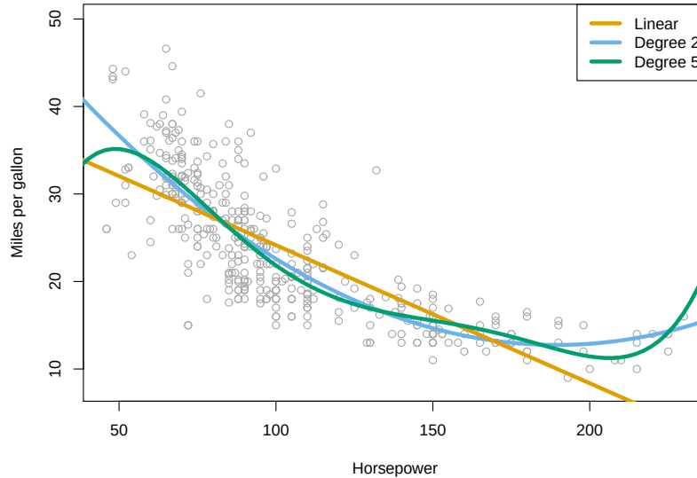
Figure 6: Polynomial regression on the Auto data. The relationship between miles per gallon and horsepower is clearly nonlinear, and polynomial terms can improve the fit.
