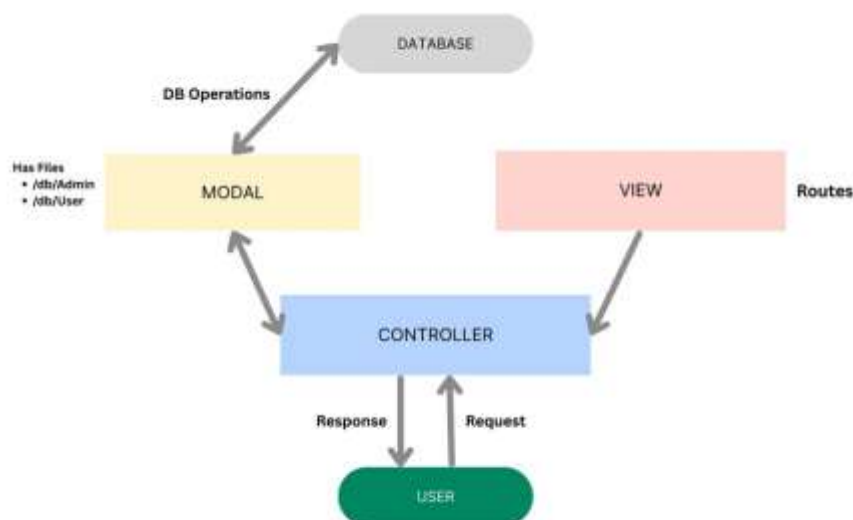
Figure 4. Enhanced user-flow / MVC representation.
