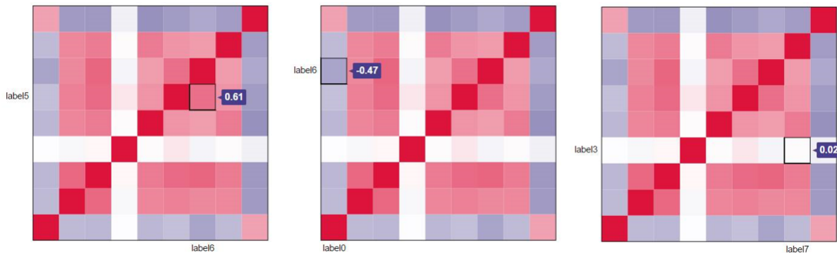
Figure 8: Correlation Matrix
