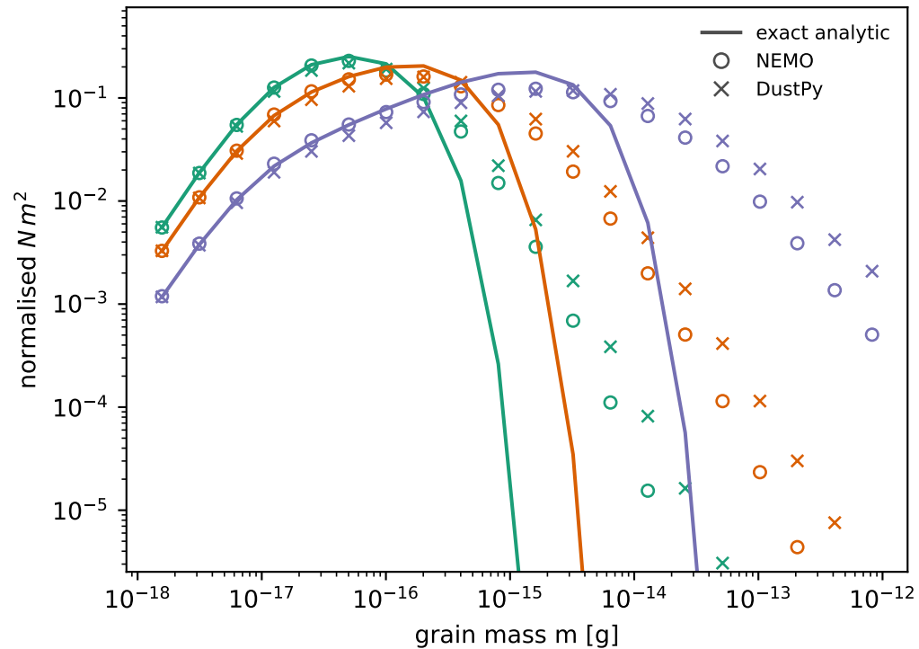
additive kernel
