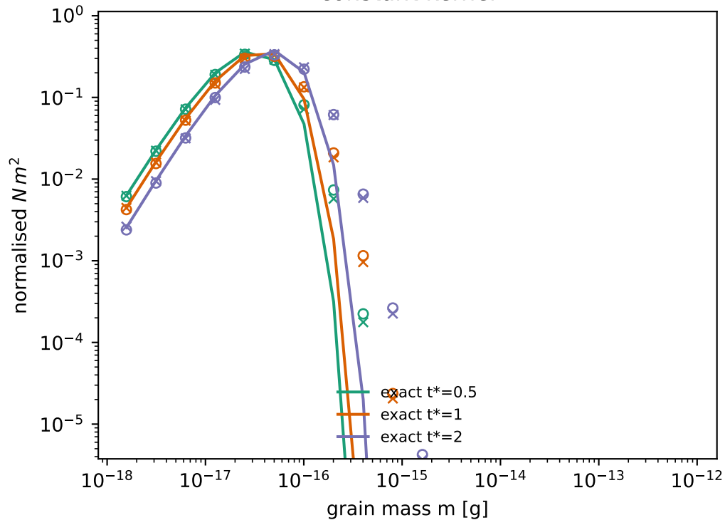
constant kernel
