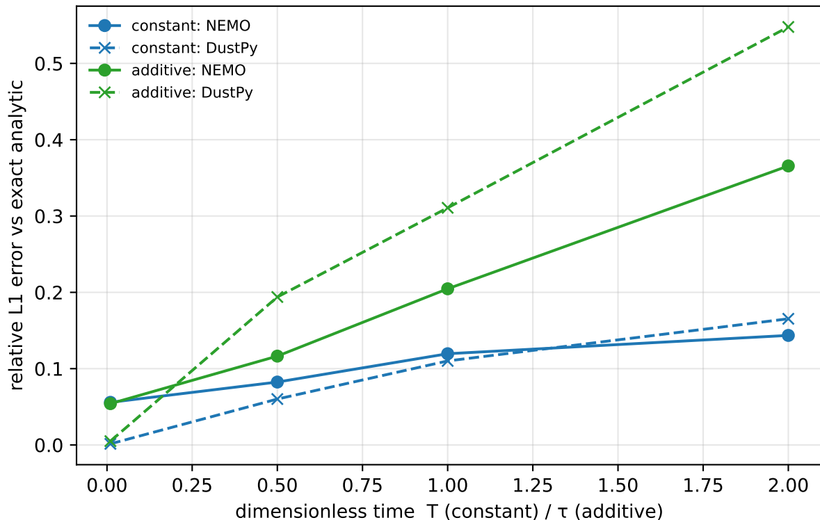
NEMO and DustPy reach the analytic to comparable error (20-bin fiducial grid, k=0 scheme both codes)
