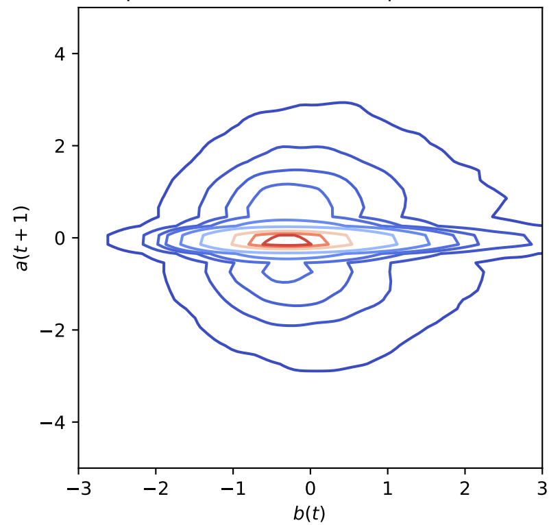
Spearman R is 0.01 with p value 0.0
