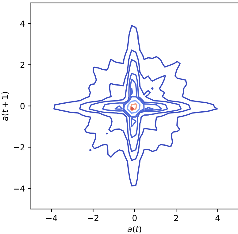
Spearman R is 0.01 with p value 0.0
