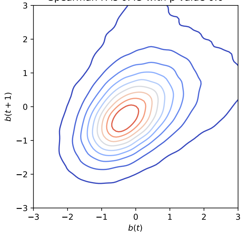
Spearman R is 0.43 with p value 0.0
