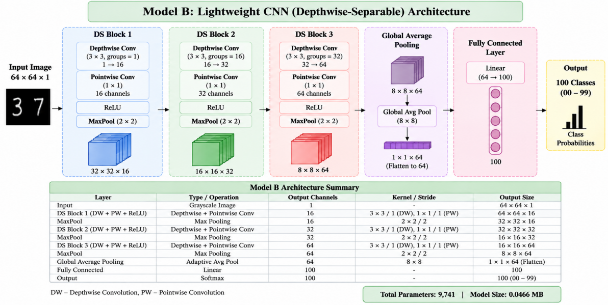
Figure 3.1: Lightweight Model
