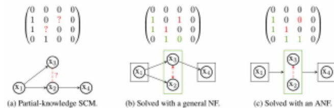
Figure: SCC reduction for partial graphs: intra-SCC modeling with preserved inter-SCC DAG.
