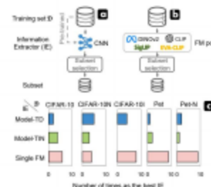
Figure: One-shot subset selection: traditional IE vs. a single FM. Our FM-based IE excels on fine-grained data.
