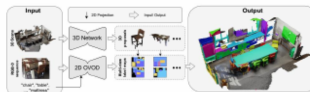
Figure: VAcc assigns top-k visible views; MVPDist aggregates labels at 2D projections to choose the class.
