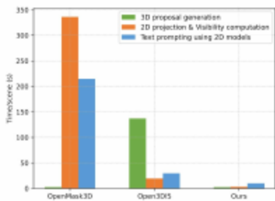
Figure: VAcc removes per-mask loops; detector-only LG maps avoid SAM overhead.
