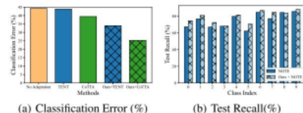
Figure: CIFAR10标签移位：现有/鲁棒TTA难适配；本框架提升召回并增强TTA
