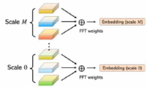
Figure: Multi-resolution: S–T mix; fuse K period reps → M scales
