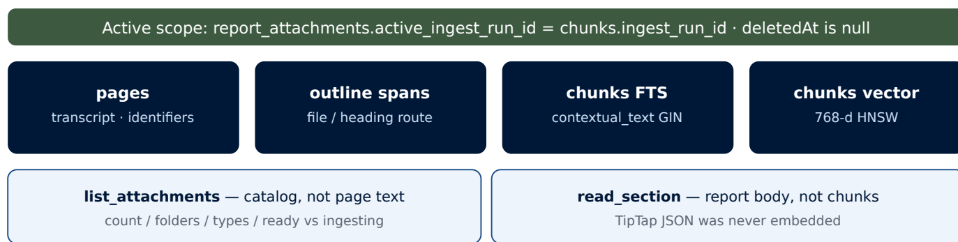
Figure 1. File-set questions use list_attachments . Which files mention a fact inside a PDF use search_documents . The report body uses read_section .
