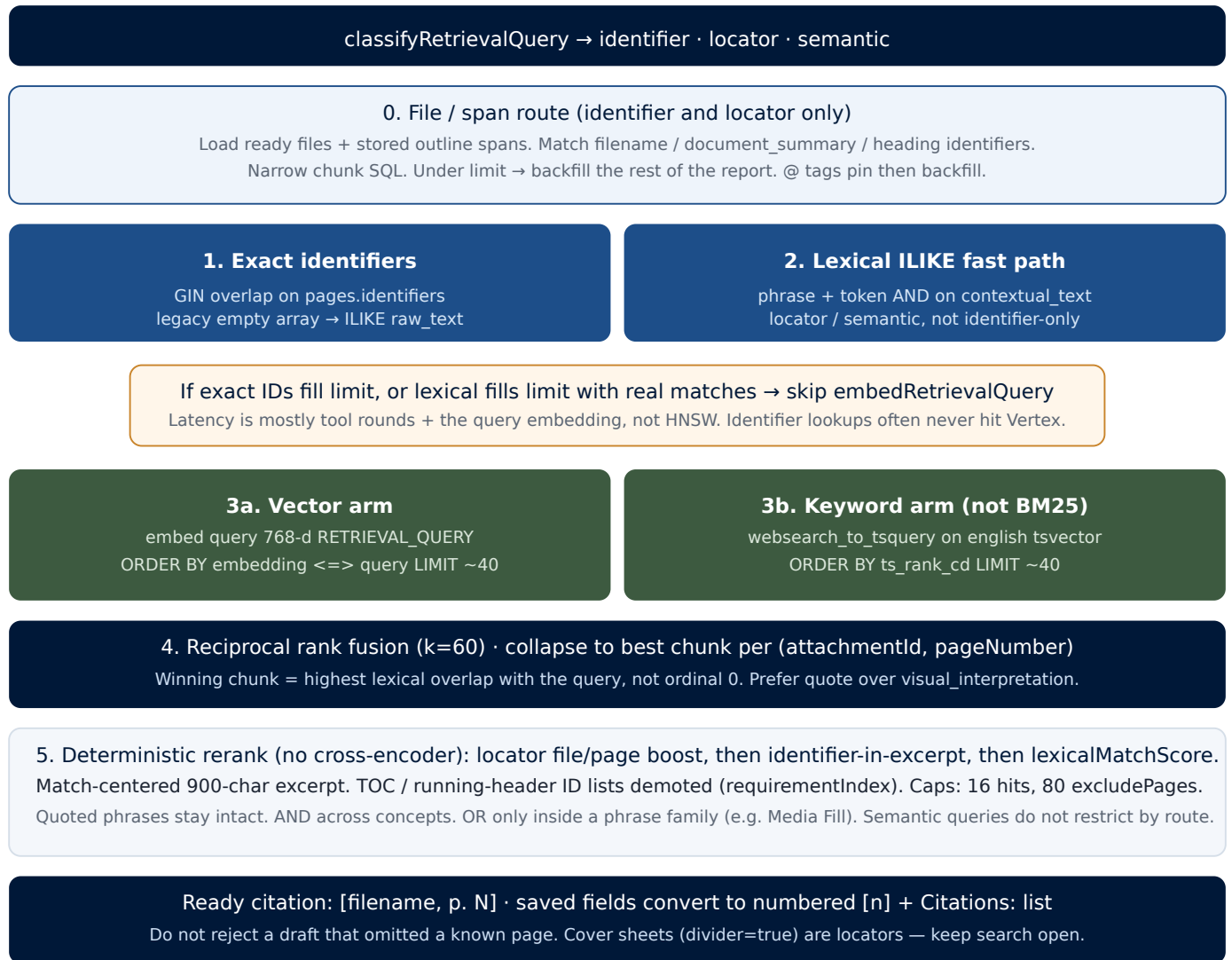
Figure 2. Two SQL lists, fused in application code. Adding Elasticsearch would duplicate this and leave the harness still deciding when to grep.
