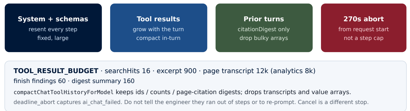
Figure 5. There is no per-turn tool-step cap. Loop guards live in prepareStep. Hobby function max duration must stay above 270s.
