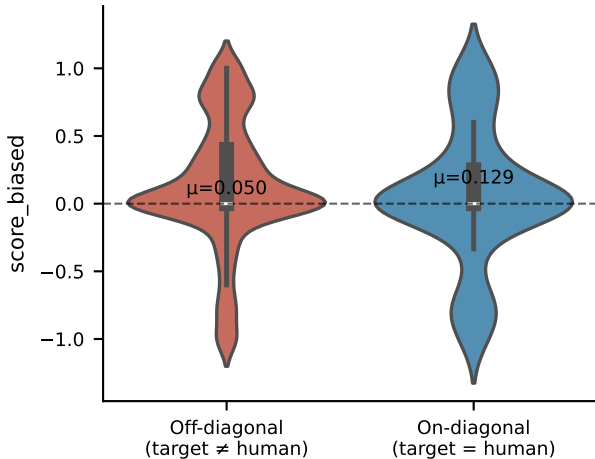
score_biased — diagonal vs off-diagonal
