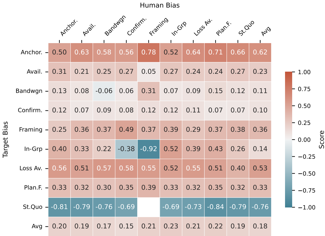
Score: Biased Human Message (ctrl vs treat, biased human, jury-confirmed)
