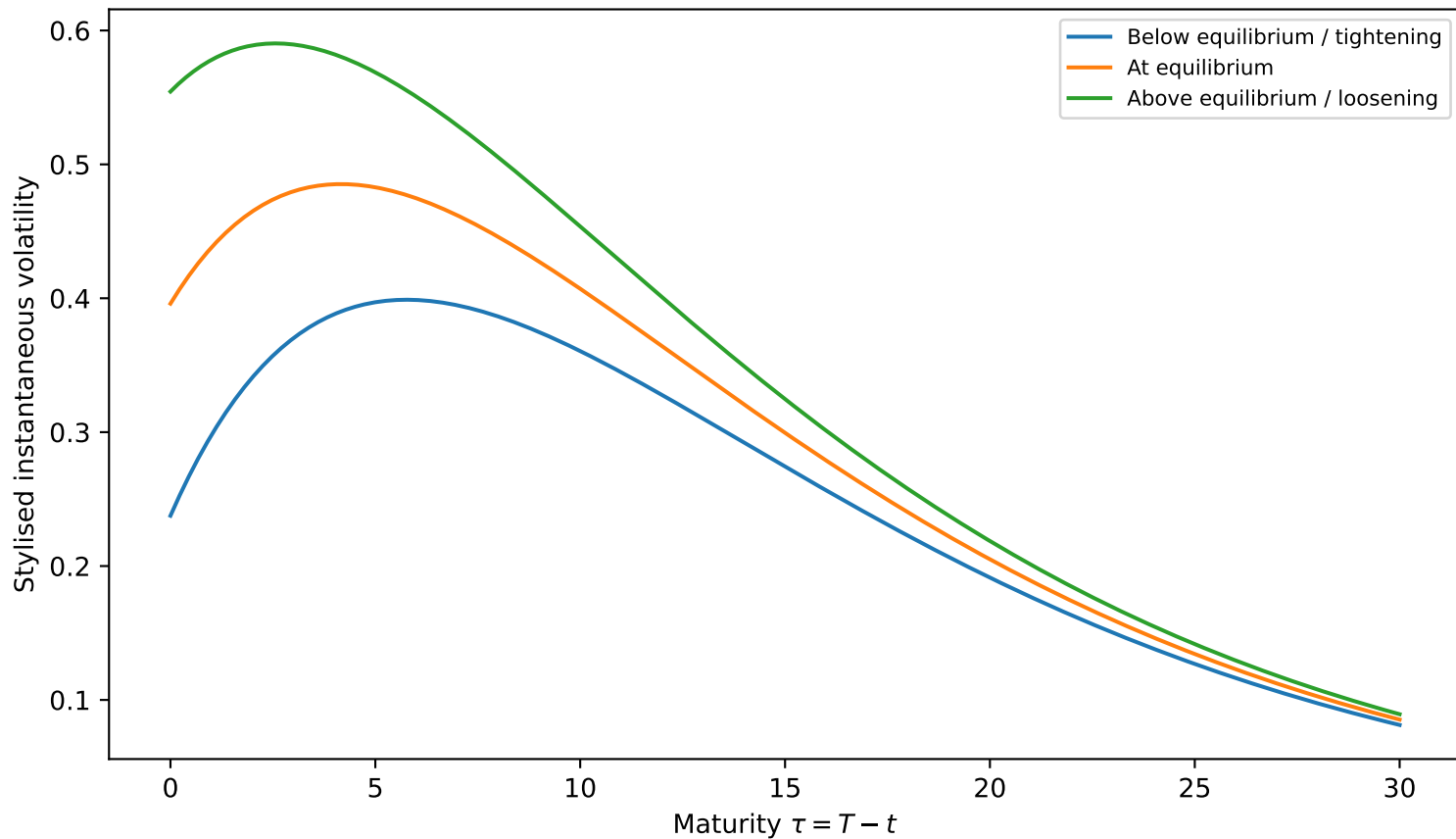
Stylised 80/20 Robin volatility curves, \chi = 1
