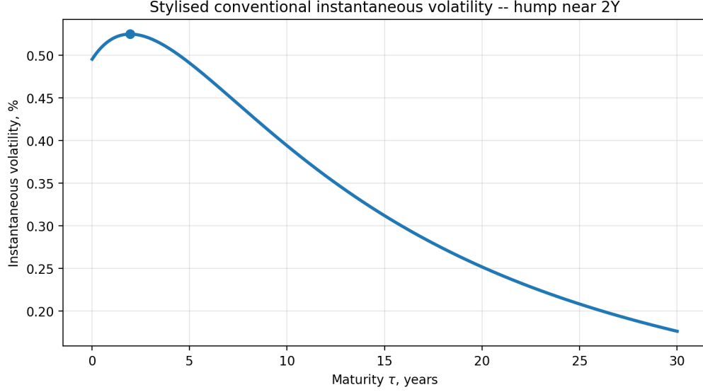
Figure 2: Stylised conventional-rate instantaneous volatility under the same parameter set. The volatility is non-zero for finite maturity and has an interior hump close to two years.
