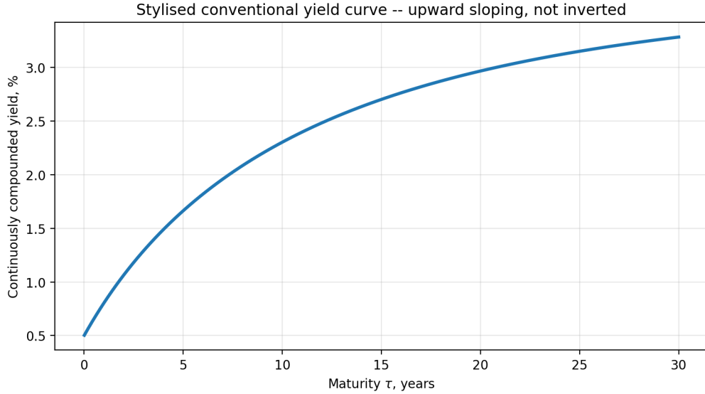
Figure 1: Stylised upward-sloping conventional yield curve under the general r -branch.
