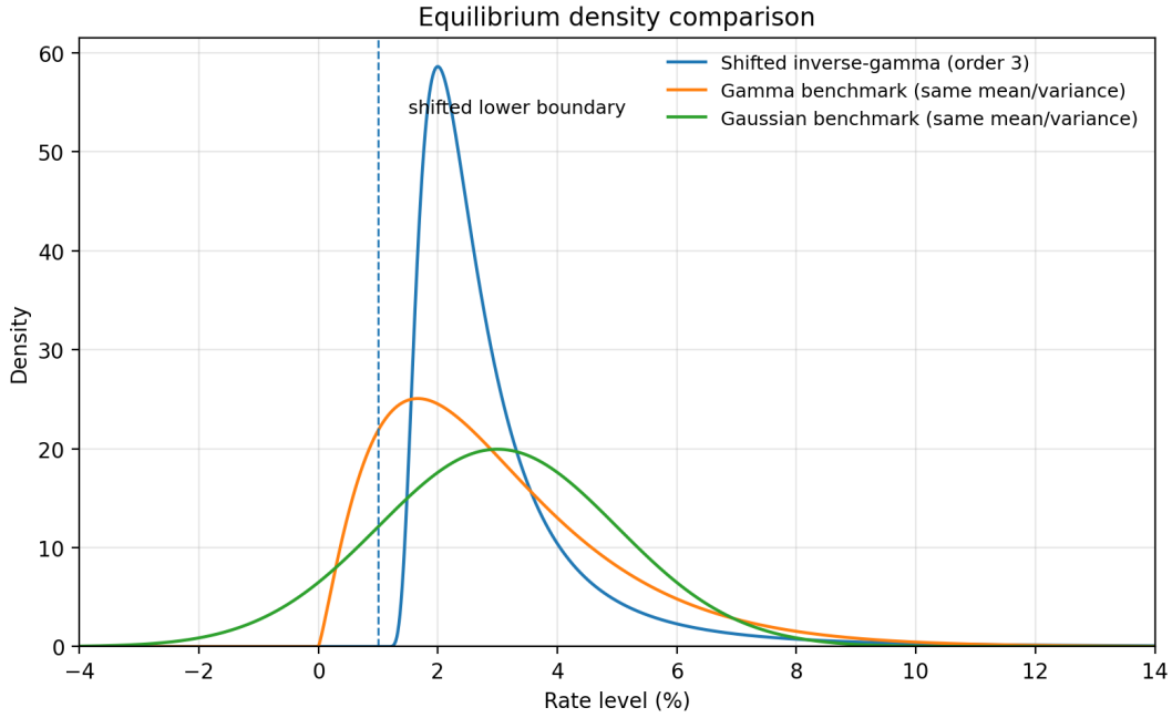
Figure 3: Comparison of equilibrium density shapes. The figure compares a shifted inverse-gamma density of order 3 with gamma and Gaussian benchmark densities calibrated to the same mean and variance. The shifted inverse-gamma law is more strongly right-skewed and more heavy-tailed than the gamma benchmark, while the Gaussian benchmark assigns probability mass to negative values. The dashed vertical line marks the shifted lower boundary.
