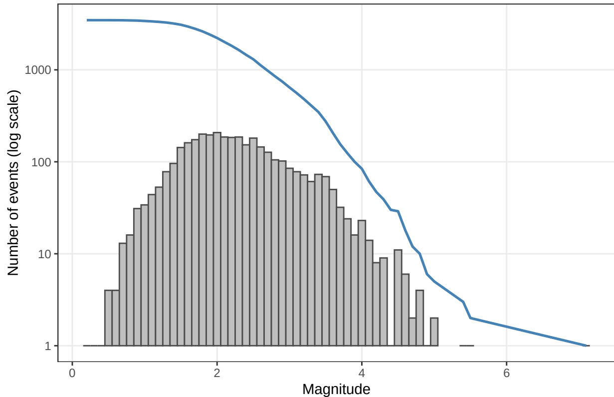
Frequency-magnitude distribution on 6 July 2019
