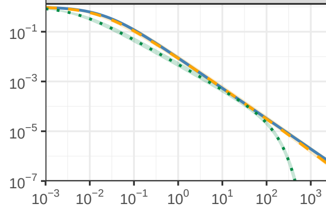
Unnormalised decay, g(t)
