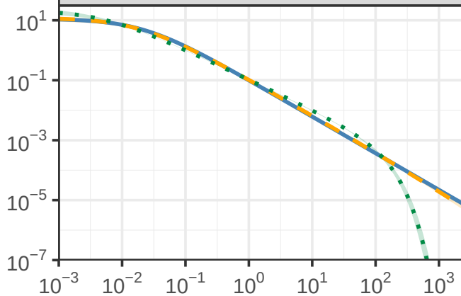
Window-normalised decay, h(t)
