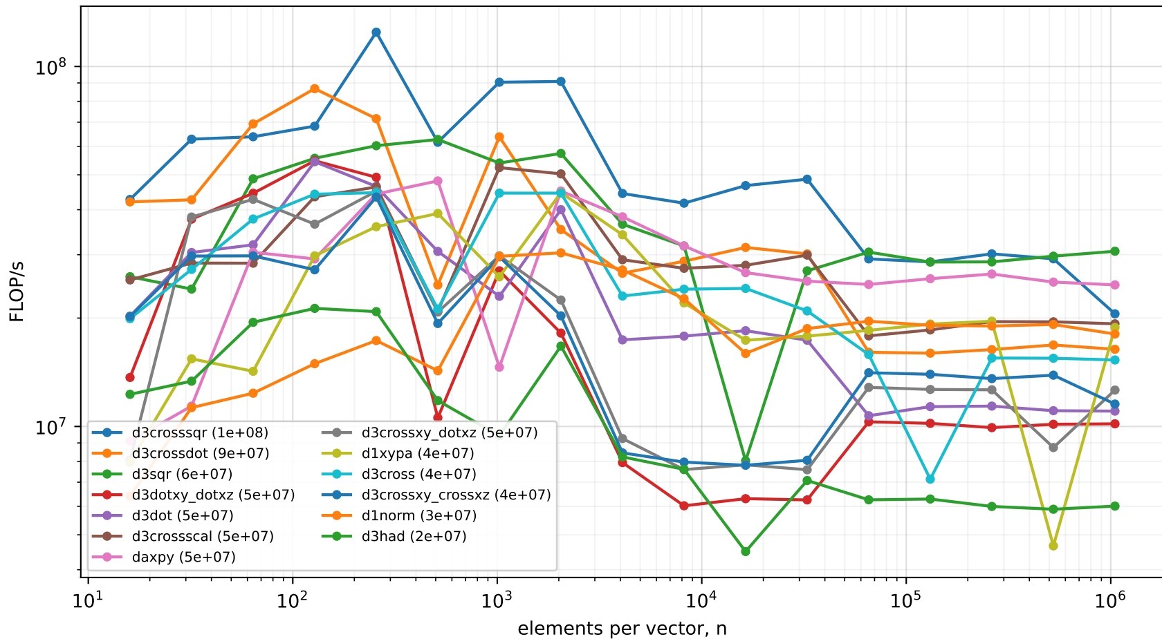
OpenBLAS physics kernels: throughput vs problem size double precision, 1 core — L2 peak at n \approx 10^2 - 10^3 , DRAM plateau from n \approx 10^5
