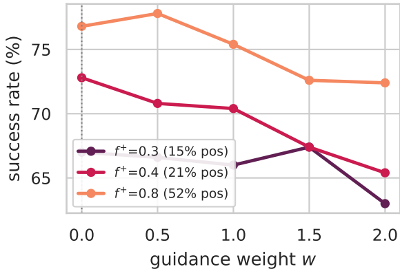
Guidance-weight sweep (LIBERO-spatial)
