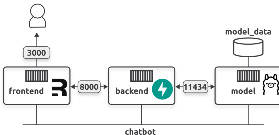
Figure9.3 - Sample app
