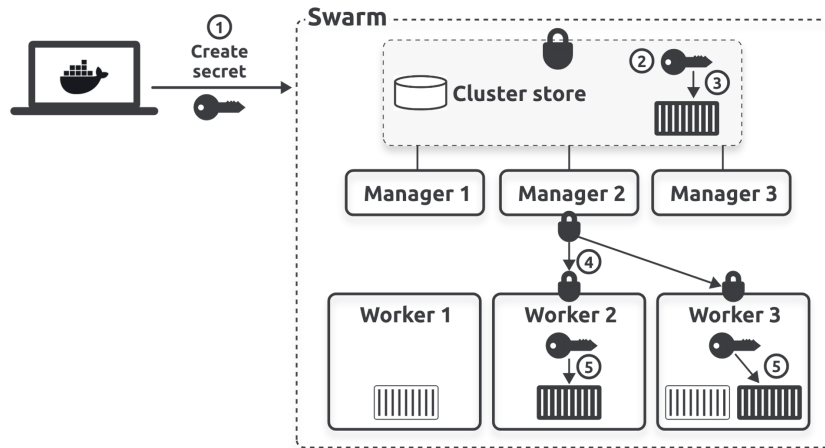
Figure 16.10 - Secret workflow
