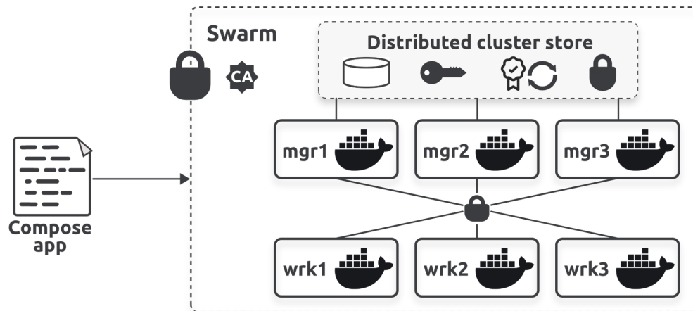
Figure 11.1 High-level swarm
