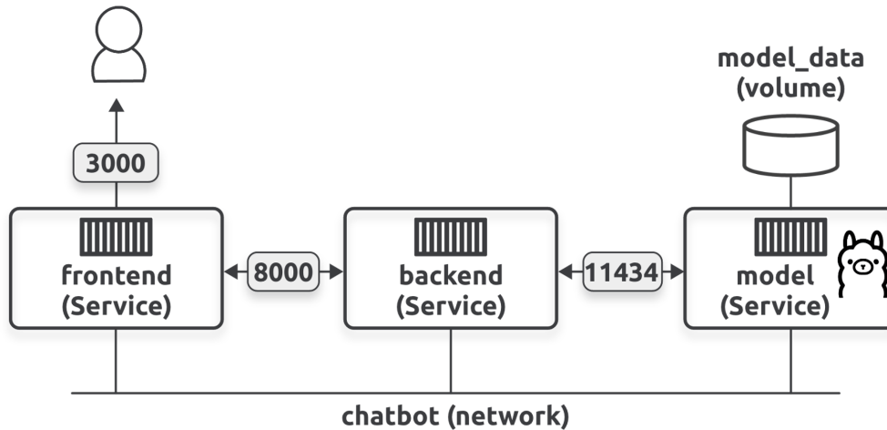
Figure9.1 - Sample app
