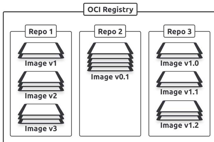
Figure 6.3 - Registry architecture
