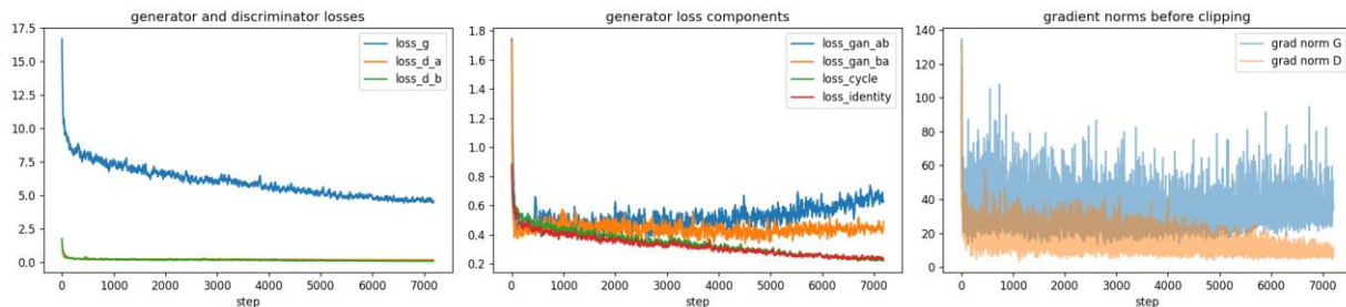
Poushali: generator and discriminator losses, loss components, and gradient norms over 7,200 steps.
