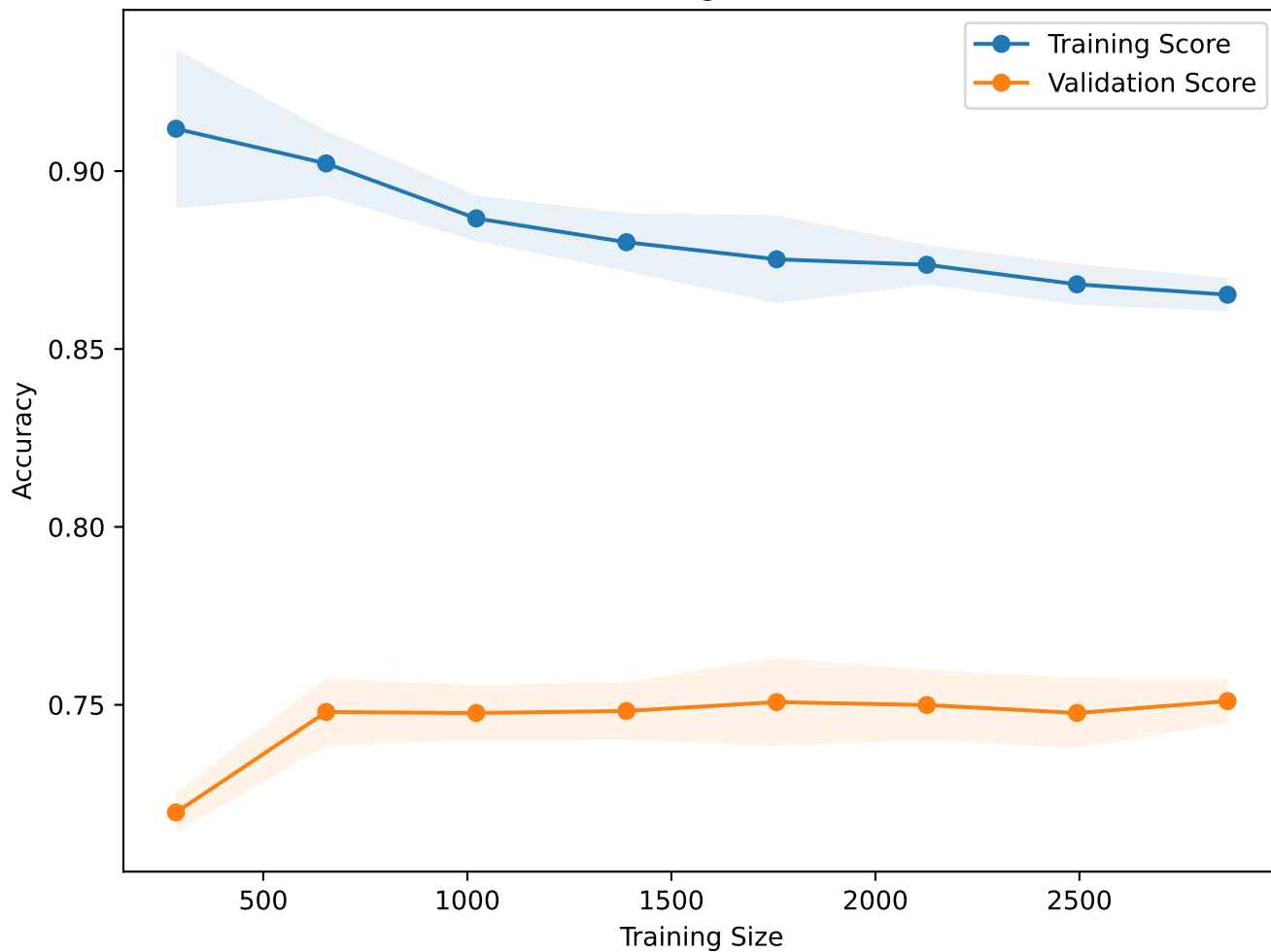
Learning Curve
