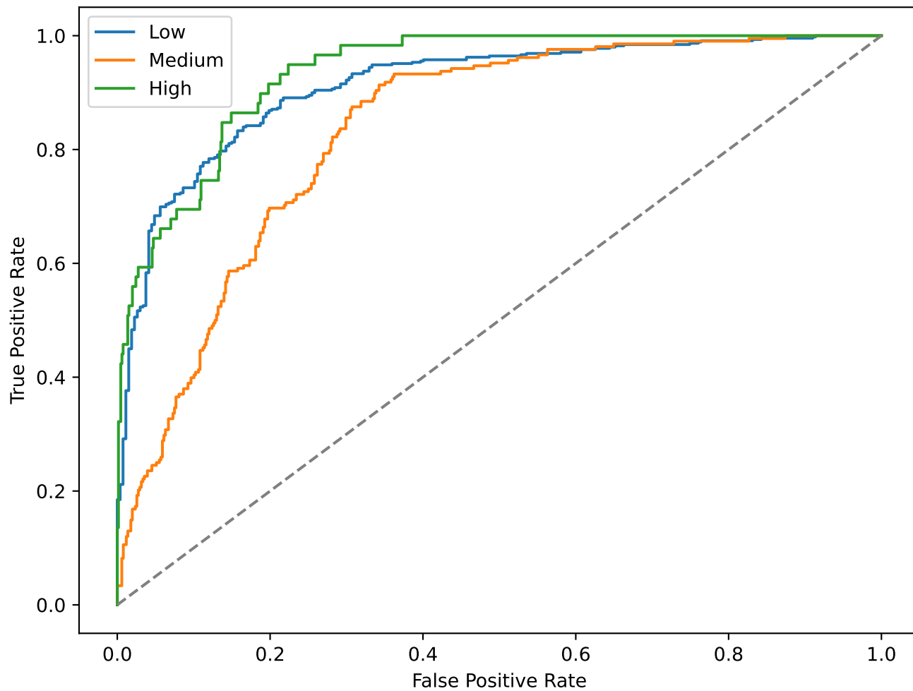
ROC Curve
