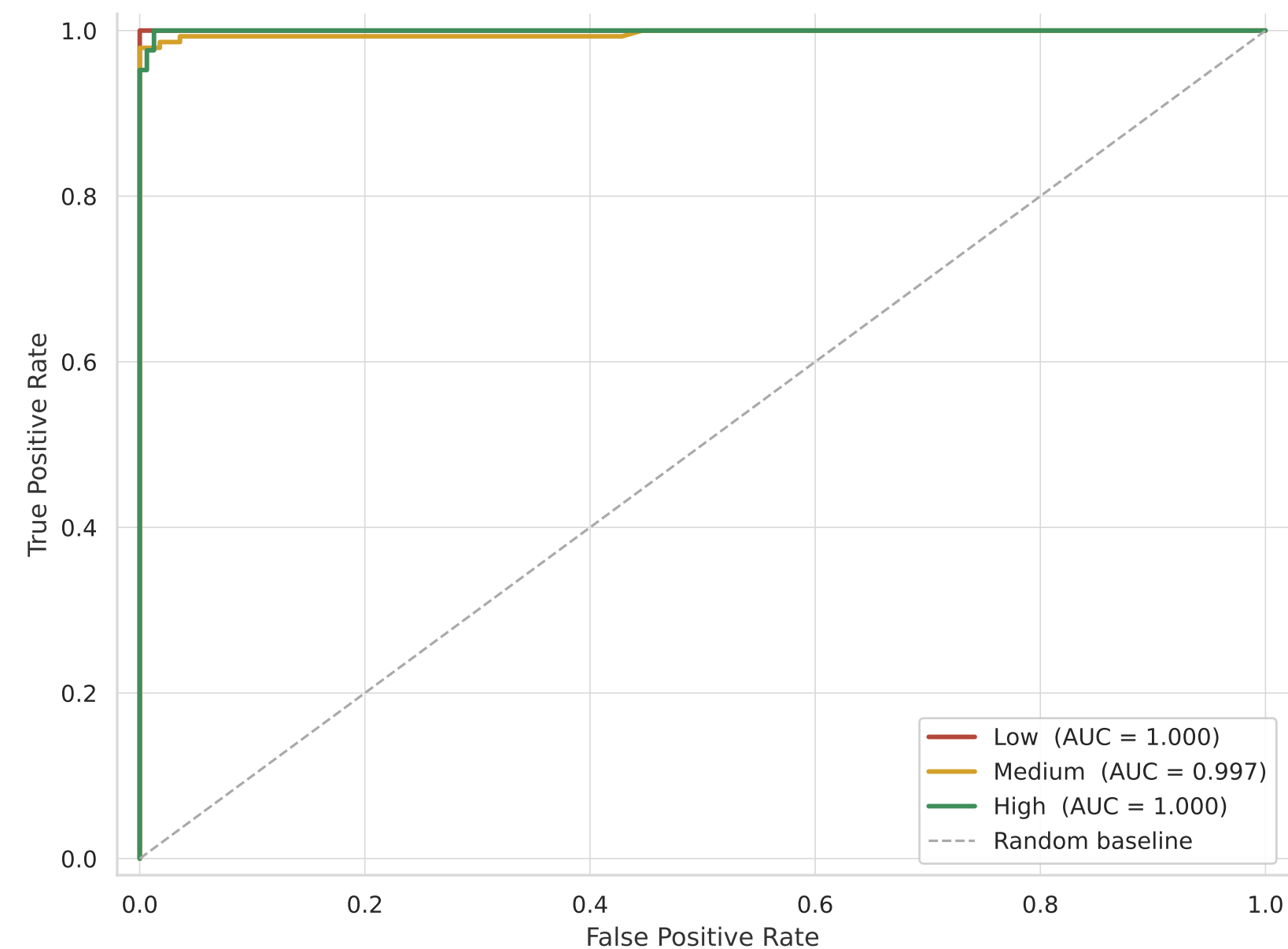
ROC Curves — One-vs-Rest by Performance Band
