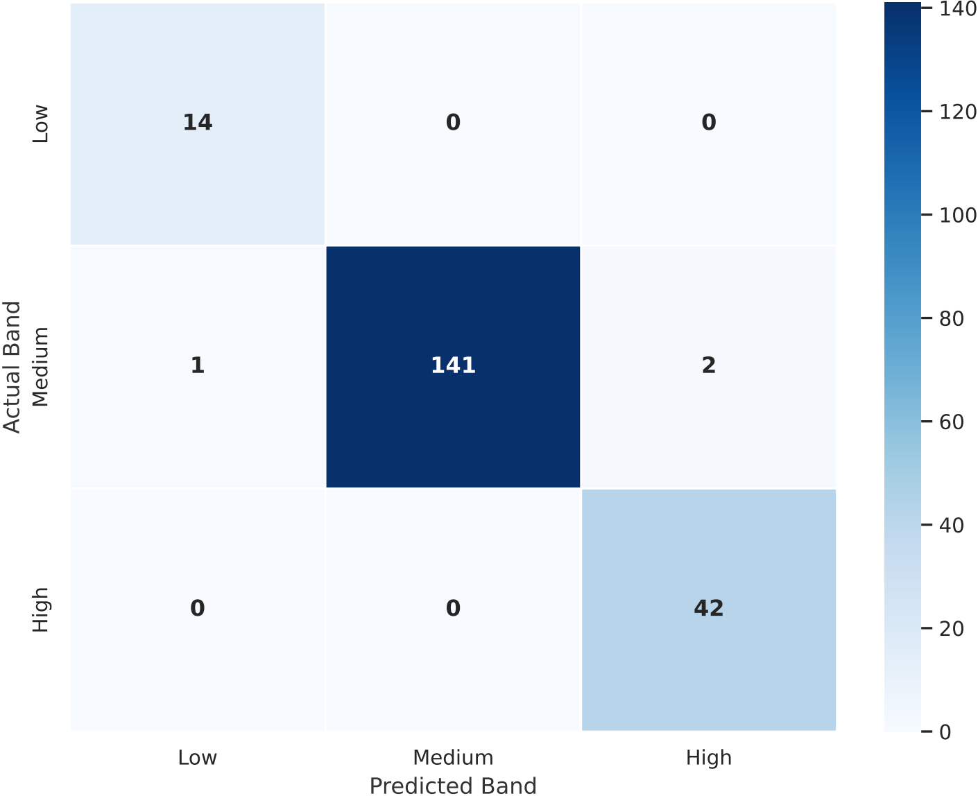
Confusion Matrix — Predicted vs. Actual
