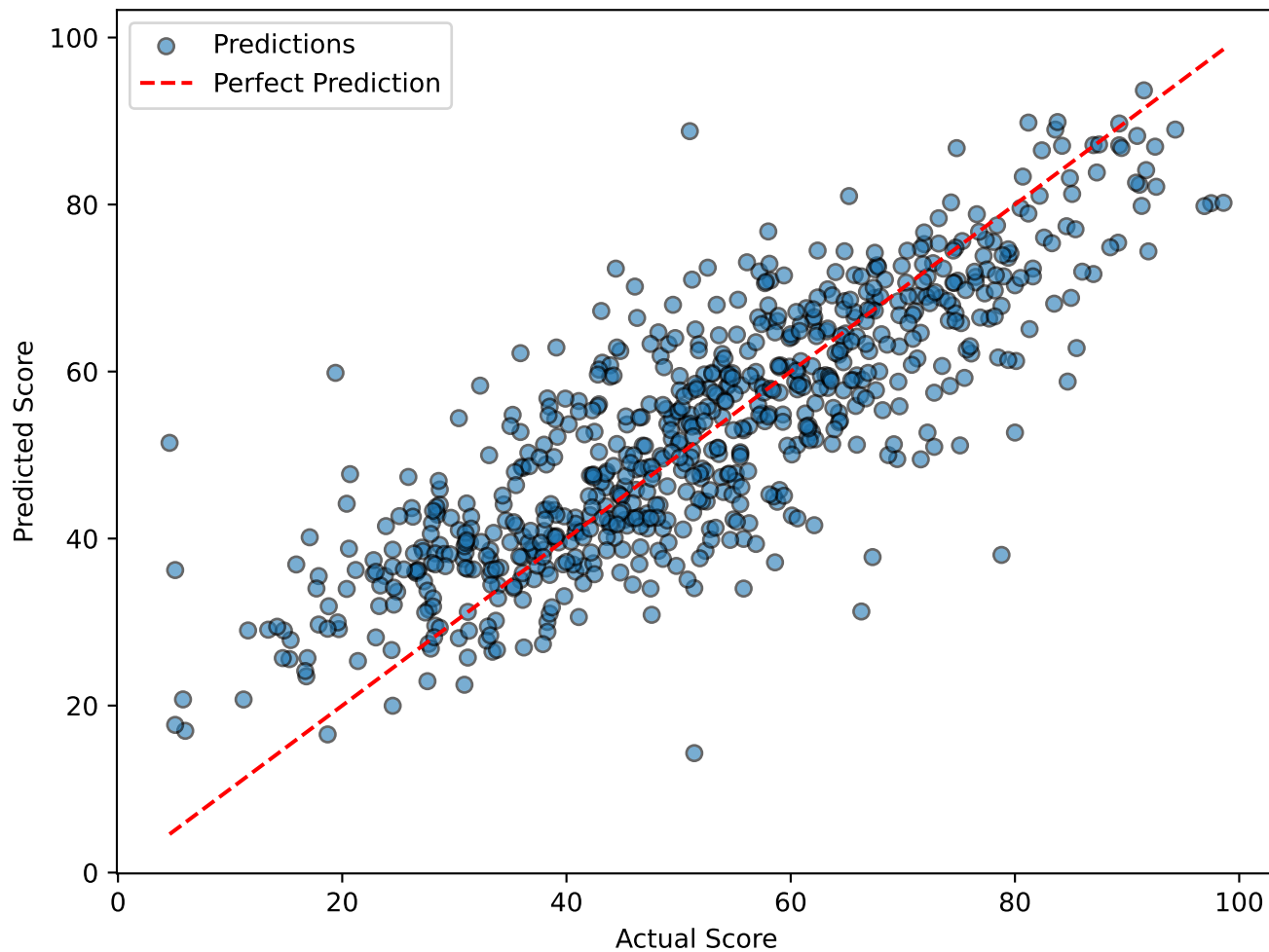
Actual vs Predicted Future Performance Score
