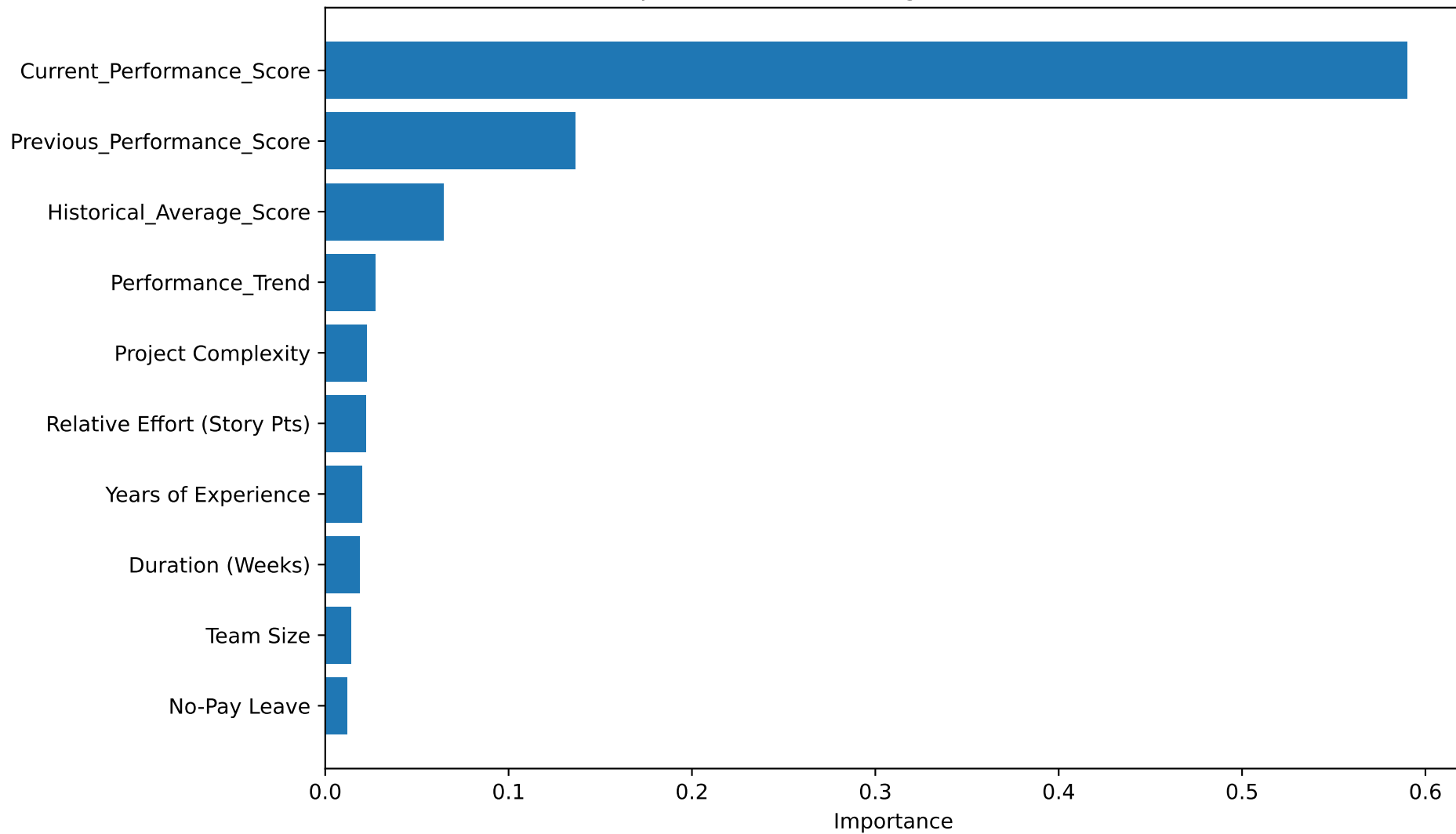
Top Features Influencing Future Performance
