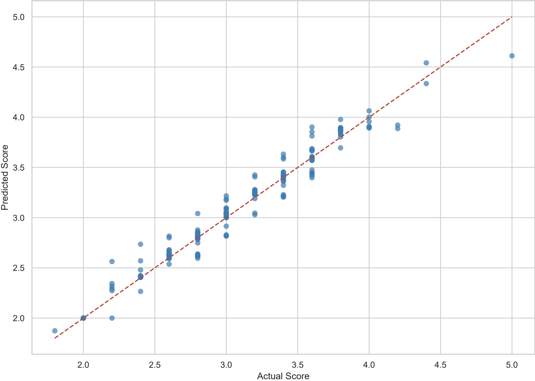
Actual vs Predicted Future Performance Score
