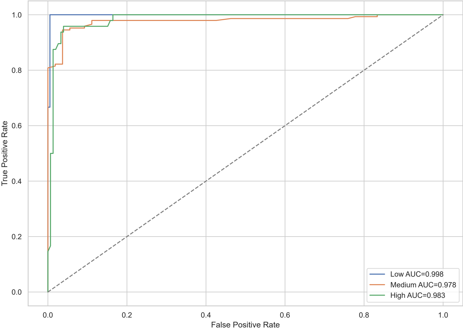
ROC Curve - Performance Classification
