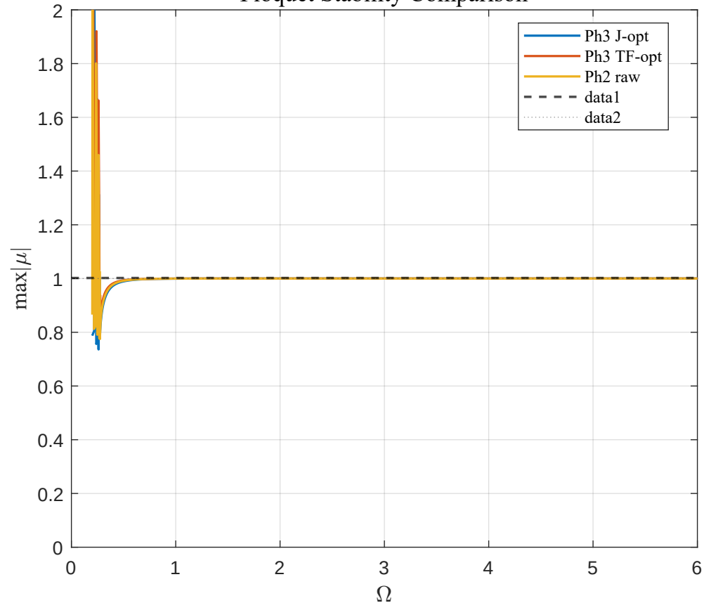
Floquet Stability Comparison
