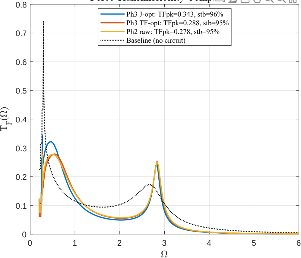
Force Transmissibility Comparison
