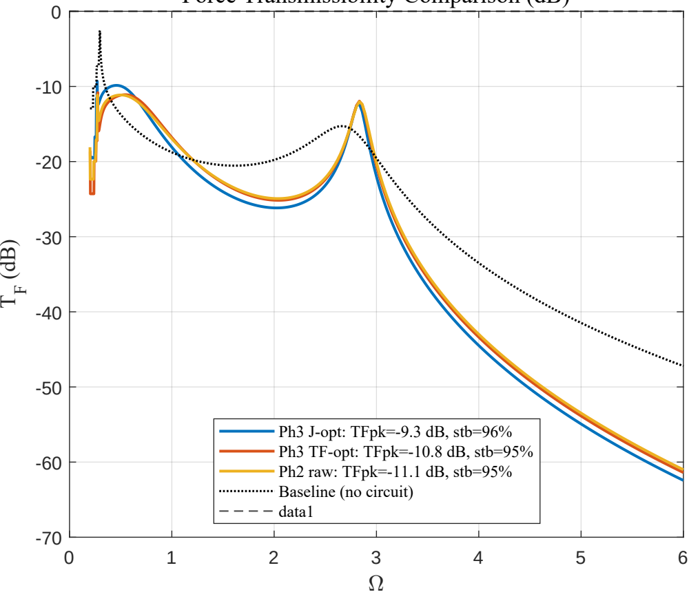
Force Transmissibility Comparison (dB)
