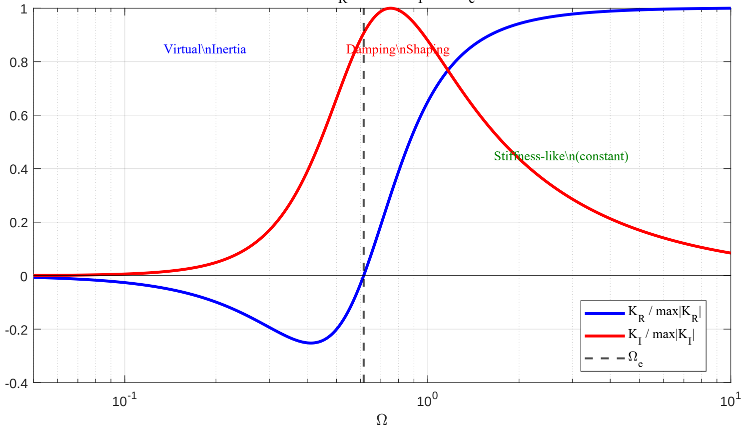
Normalized K_R(\Omega) and K_I(\Omega) , \Omega_e=0.614
