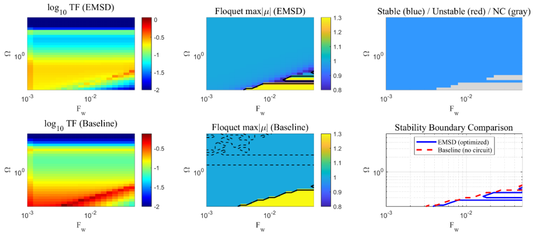
Stability Boundary Map in (F_w, \Omega) Plane EMSD: \sigma=1.1506, \kappa_c=1.5222, \kappa_c=0.5743
