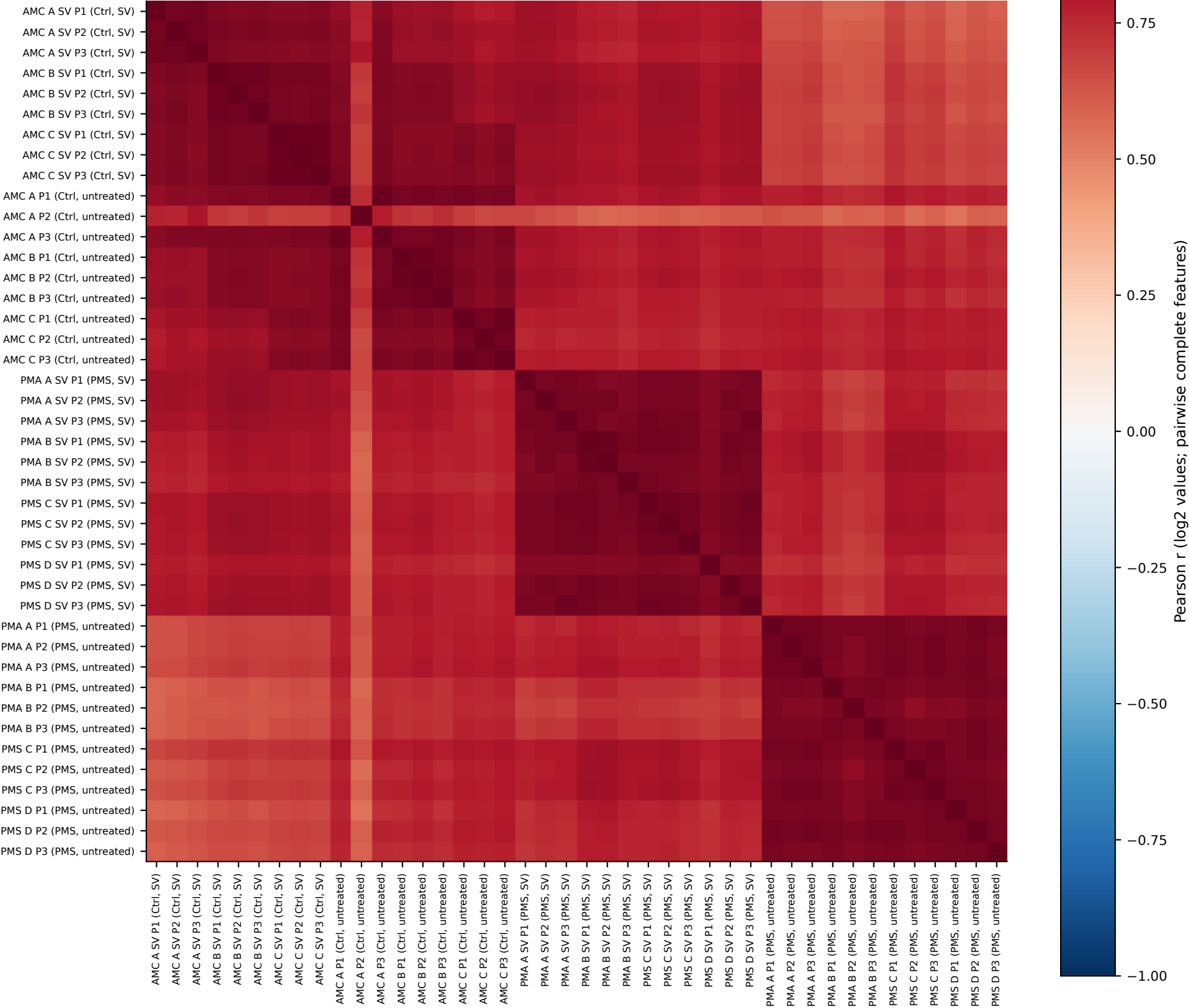
Exploratory replicate correlation — ST003328
