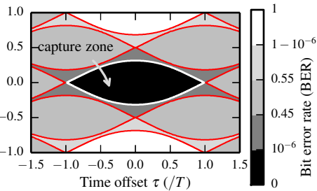
(a) Bit error rate for uncoded transmissions.
