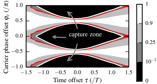
(c) Symbol error rate for DSSS/SDD.
