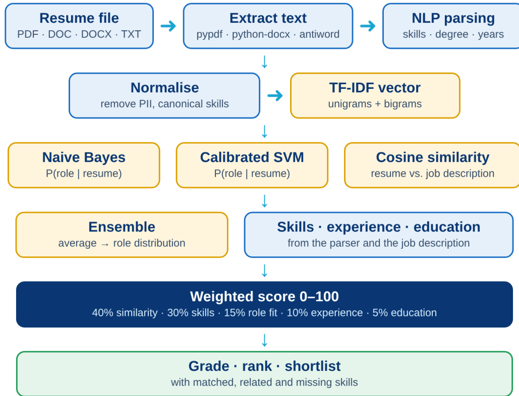
Figure 4.2 — ML Scoring Pipeline Data Flow
