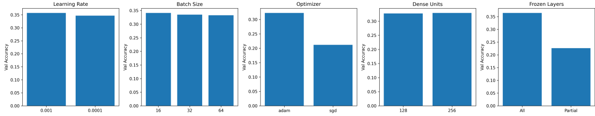
Figure 10: Validation accuracy across different hyperparameter settings (3-epoch quick comparisons).
