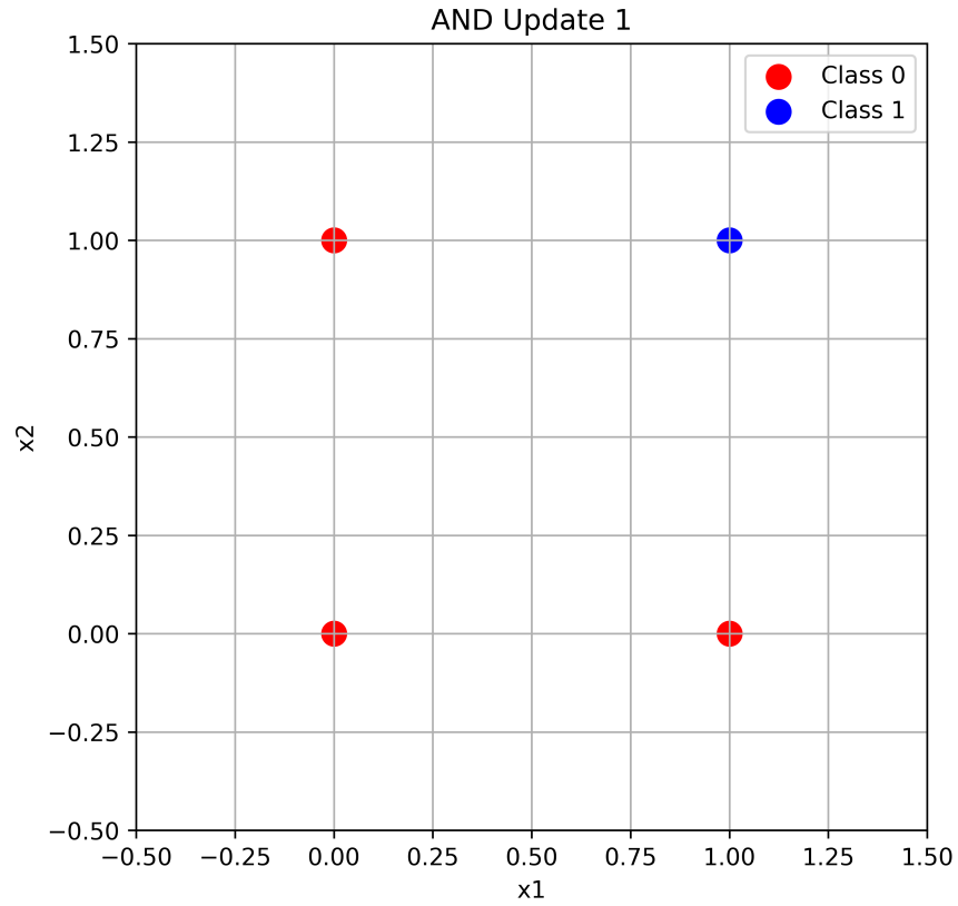
Figure 10: AND Gate Decision Boundary after First Weight Update
