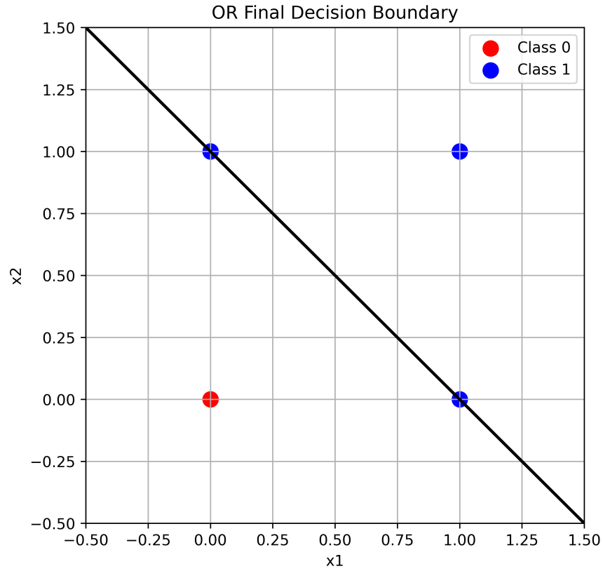
Figure 9: Final Decision Boundary for OR Gate
