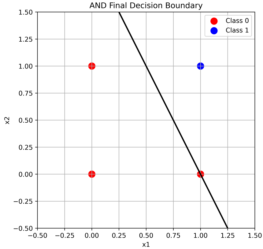
Figure 11: Final Decision Boundary for AND Gate
