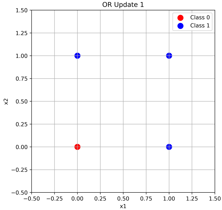
Figure 8: OR Gate Decision Boundary after First Weight Update
