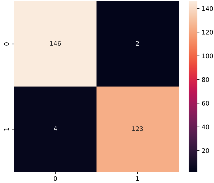
Figure 6: Confusion Matrix
