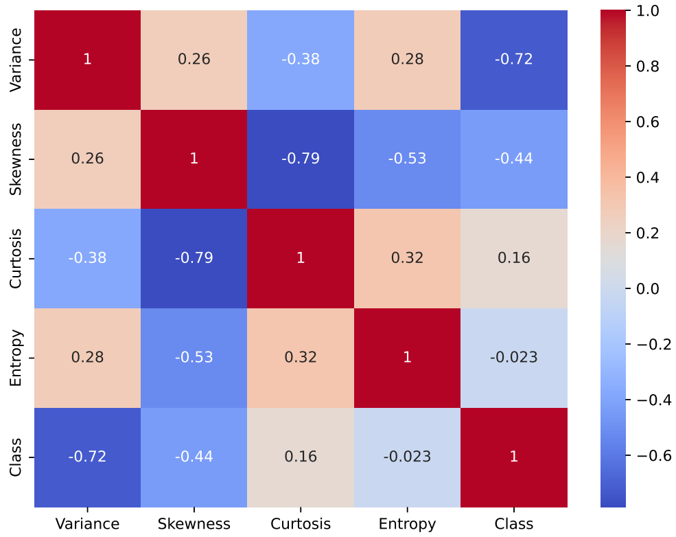
Figure 2: Correlation Heatmap
