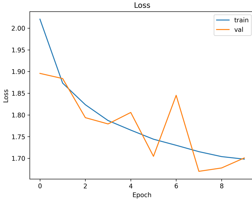
Figure 5: Training and validation loss over epochs (frozen base).
