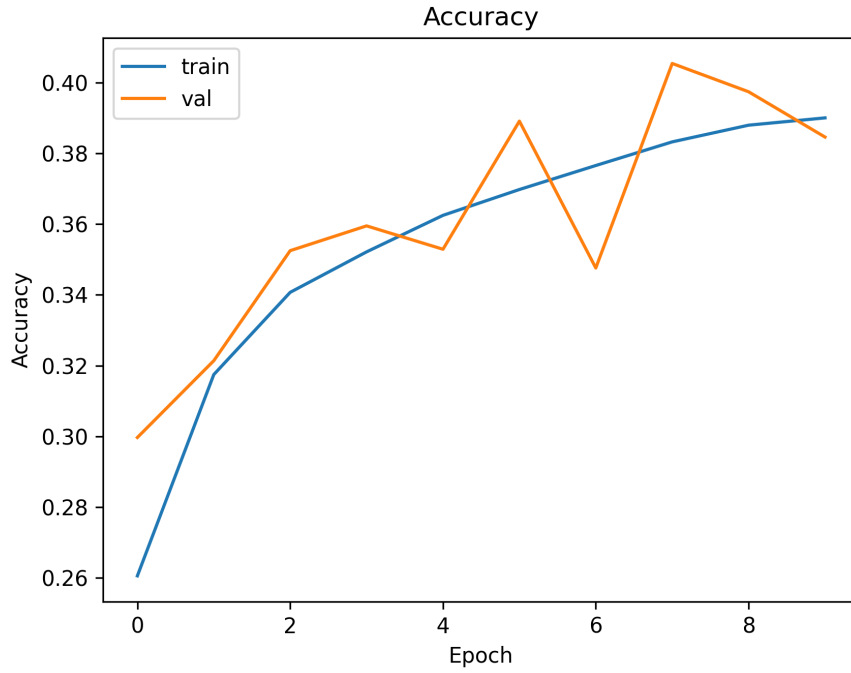
Figure 4: Training and validation accuracy over epochs (frozen base).
