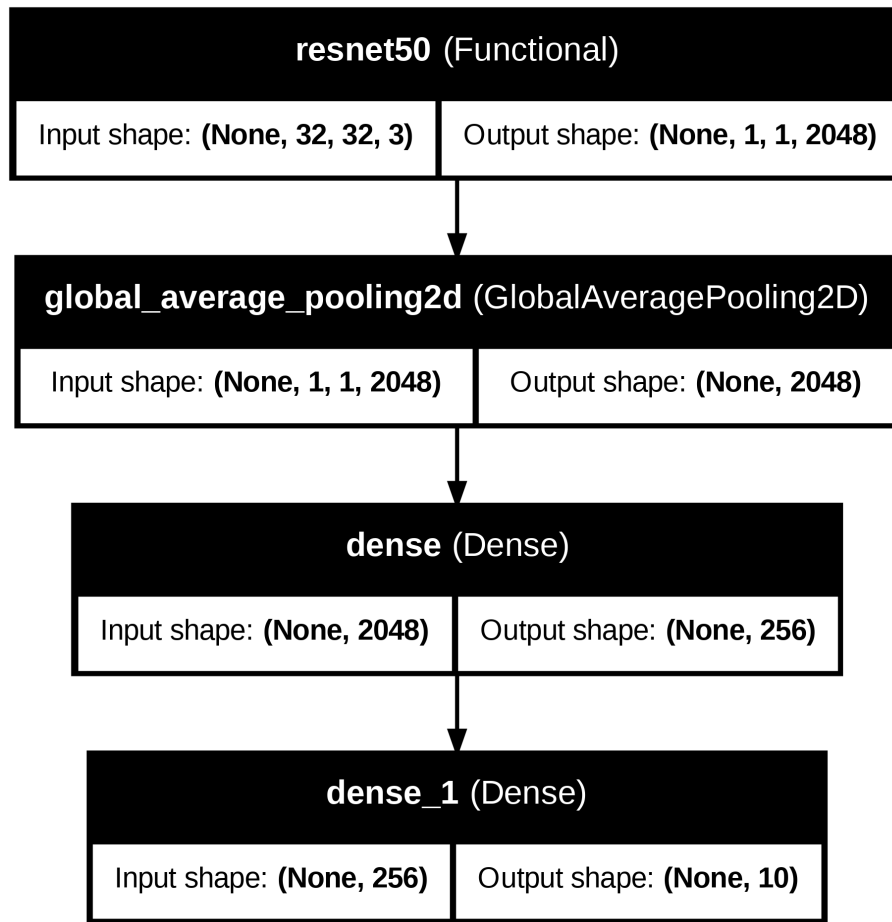
Figure 3: Transfer learning architecture built on top of the frozen ResNet50 base.
