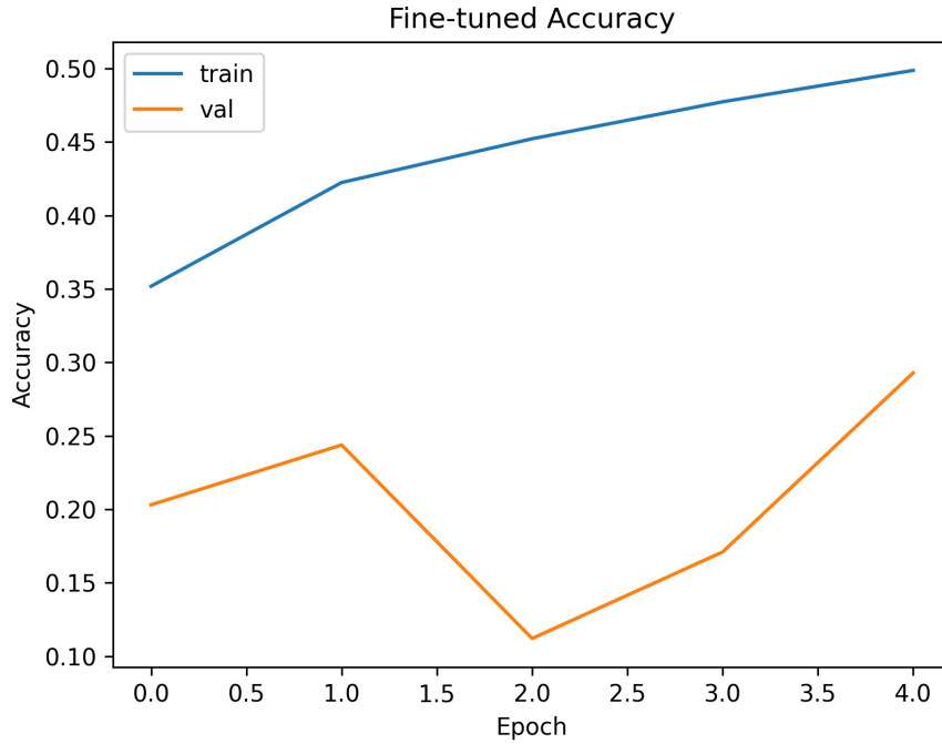
Figure 6: Training and validation accuracy after fine-tuning.
