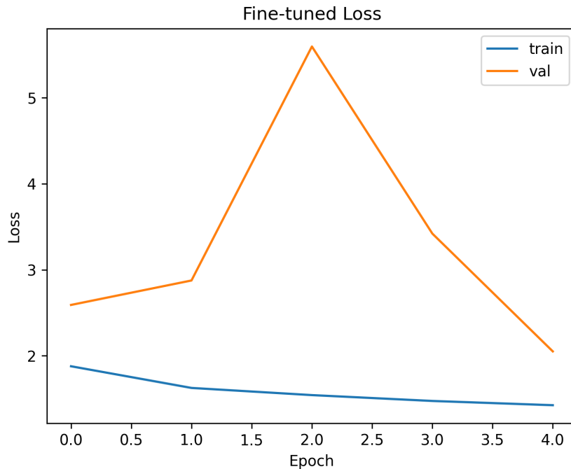
Figure 7: Training and validation loss after fine-tuning.
