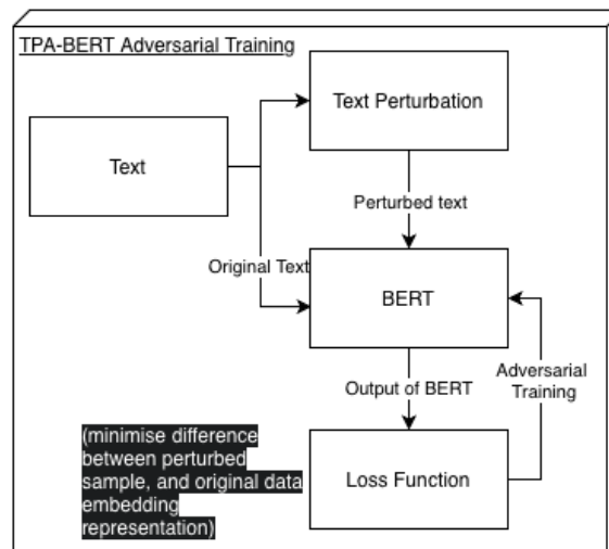
Figure 4.8: Proposed Fine-Tuning Process for TPA-BERT
