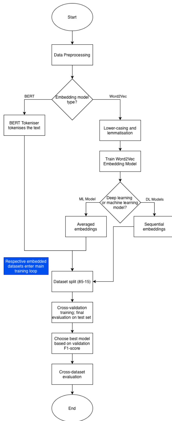
Figure 4.9: Training process from end-to-end
