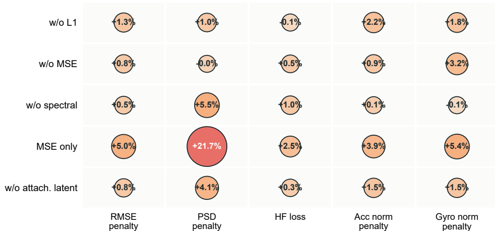
a Ablation impact fingerprint Cell value = directional performance loss relative to the full model
