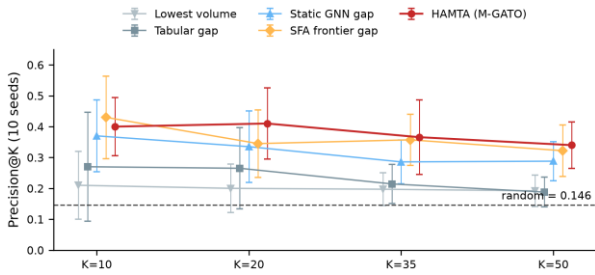
Fig. 5. Opportunity recovery precision ( Precision@K ) across marketing campaign budgets K in \{10, 20, 35, 50\} comparing HAMTA with frontier and heuristic baselines (10 random seeds, mean \pm std).
