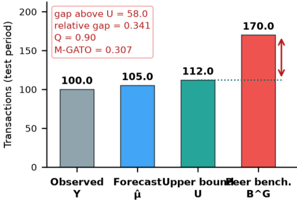
Fig. 3. Pedagogical walkthrough of the M-GATO score formulation: actual transaction volume Y , model forecast \hat{\mu} , calibrated upper natural bound U , and conservative peer benchmark B^*G .
