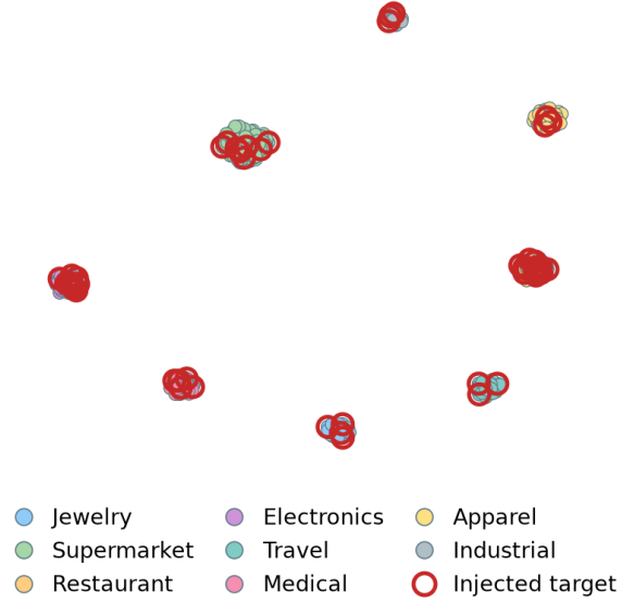
Fig. 2. Two-dimensional projection of merchant peer embeddings across eight business categories; red node rings indicate injected opportunity target merchants.
