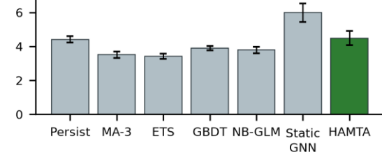
(a) Forecasting MAE (lower is better)
