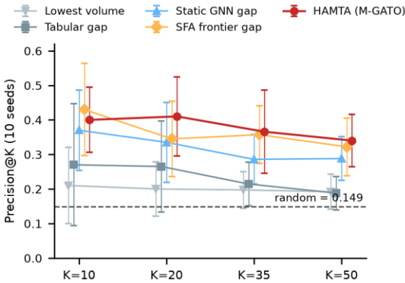
Fig. 5. Opportunity recovery precision ( \text{Precision}@K ) across marketing campaign budgets K in \{10, 20, 35, 50\} comparing HAMTA with frontier and heuristic baselines (10 random seeds, mean \pm std).
