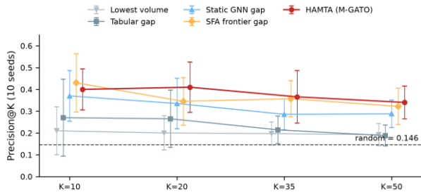
Fig. 5. Opportunity recovery precision ( \text{Precision}@K ) across marketing campaign budgets K in \{10, 20, 35, 50\} comparing HAMTA with frontier and heuristic baselines (10 random seeds, mean \pm std).
