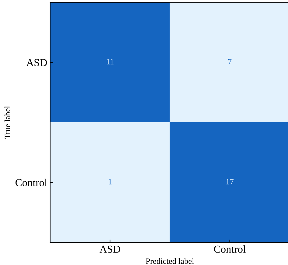
Confusion Matrix (GaussianNB)
