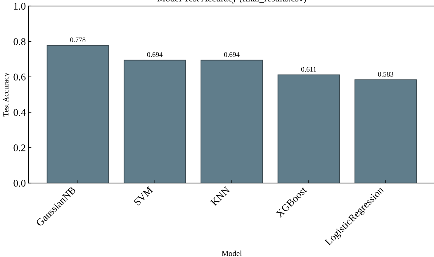
Model Test Accuracy (final_results.csv)
